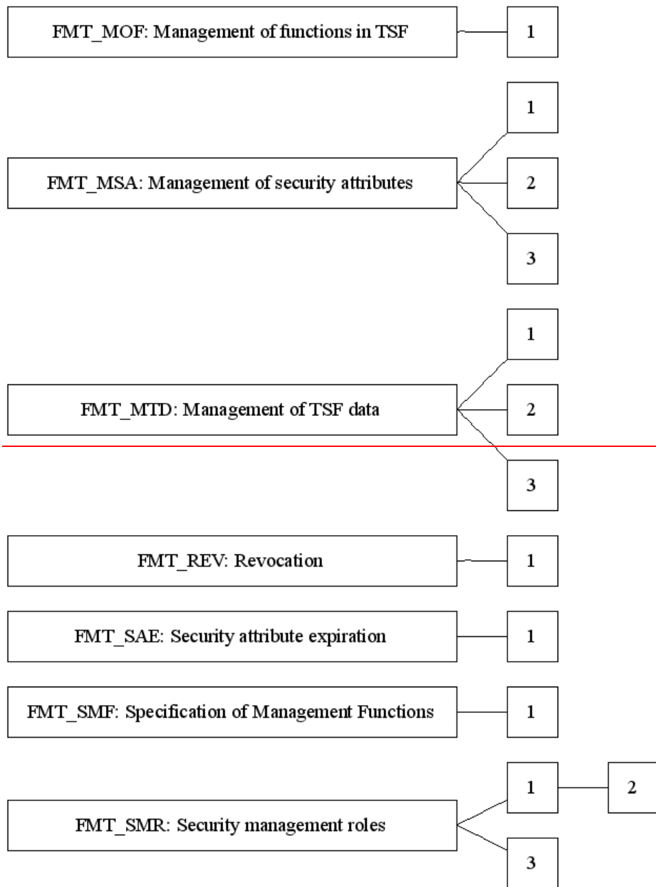
Figure 12 - FMT: Security management class decomposition
