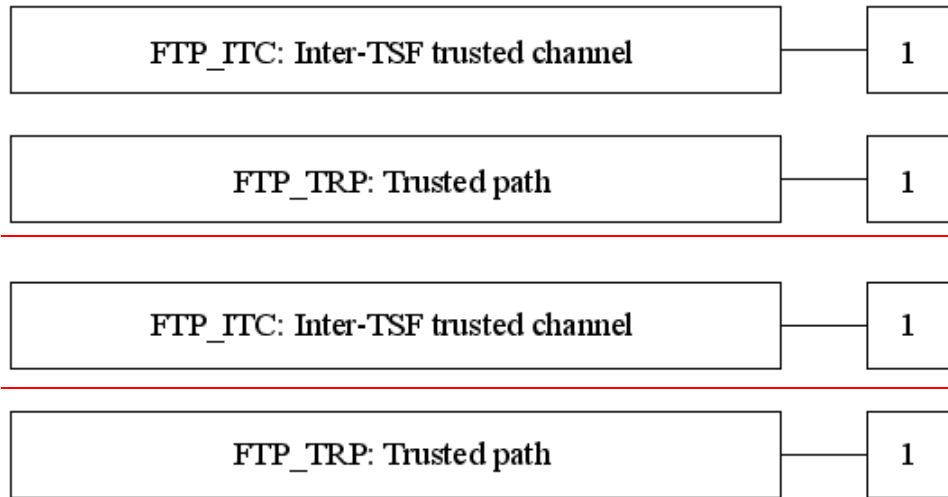
Figure 31 - FTP: Trusted path/channels class decomposition
