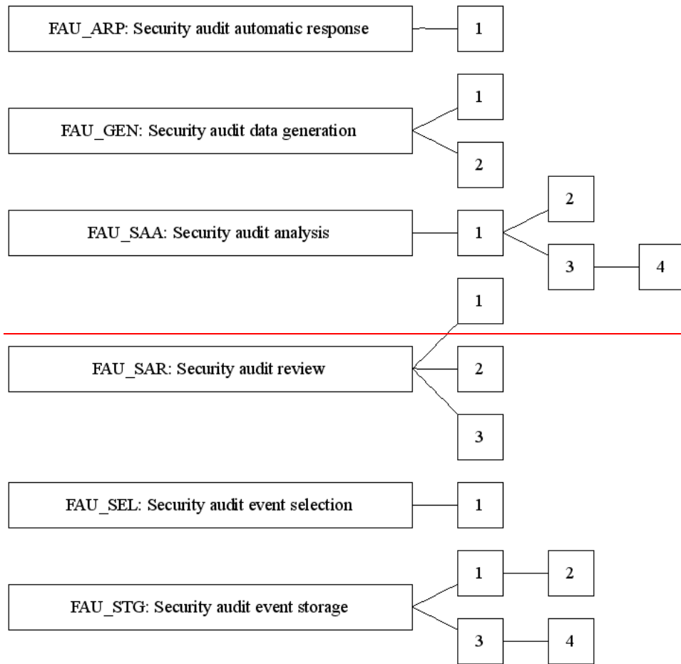
Figure 21 - FAU: Security audit class decomposition
