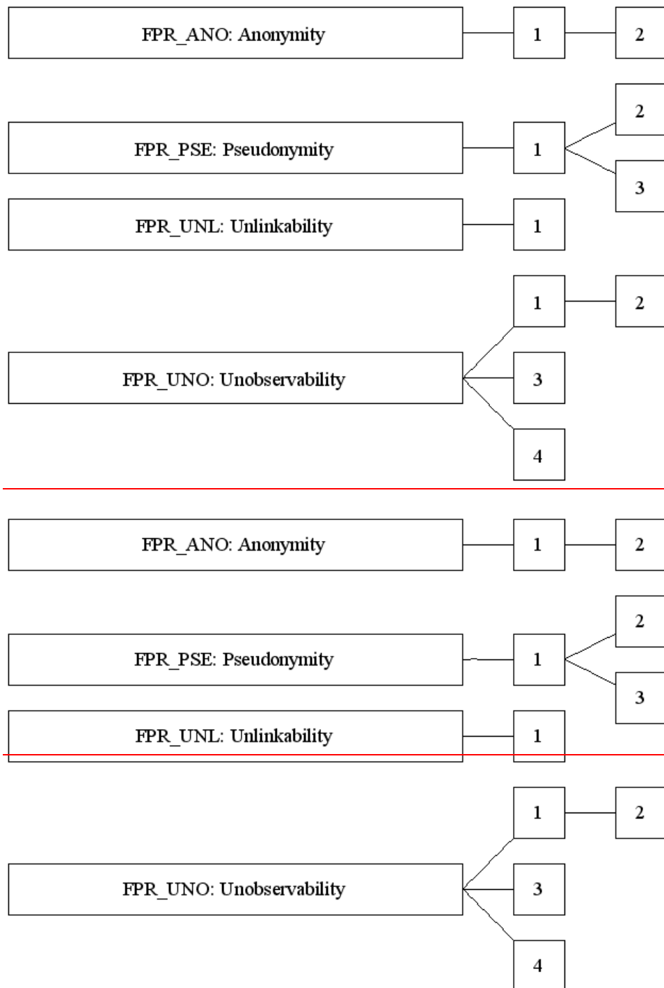
Figure 27 - FPR: Privacy class decomposition
