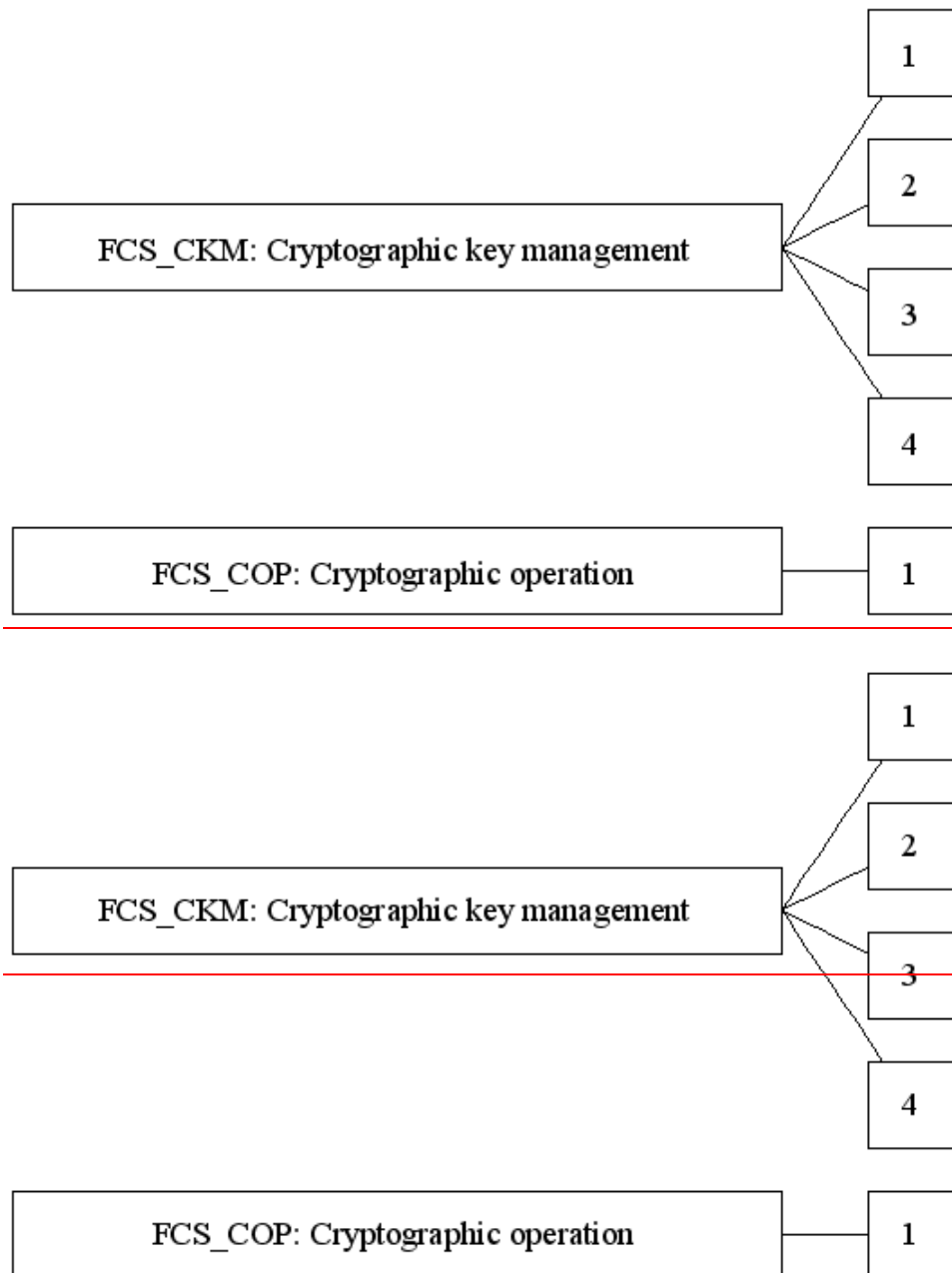
Figure 23 - FCS: Cryptographic support class decomposition
