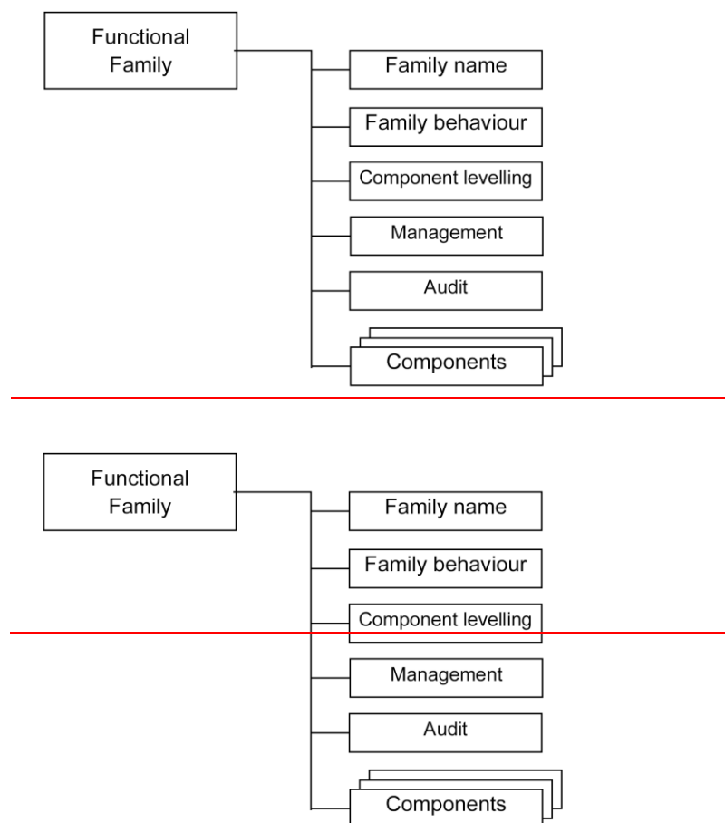
Figure 4 - Functional family structure
