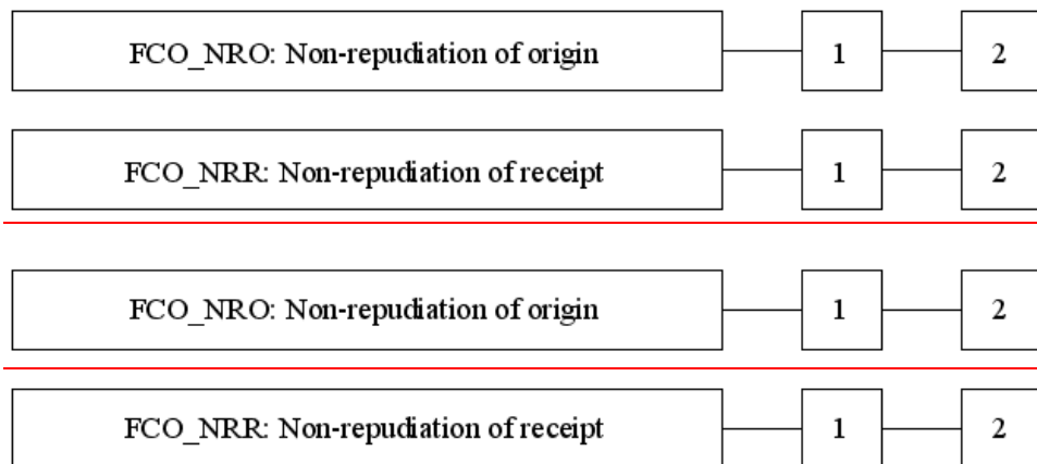
Figure 22 - FCO: Communication class decomposition
