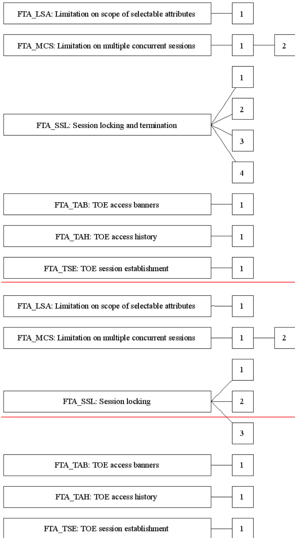
Figure 30 - FTA: TOE access class decomposition
