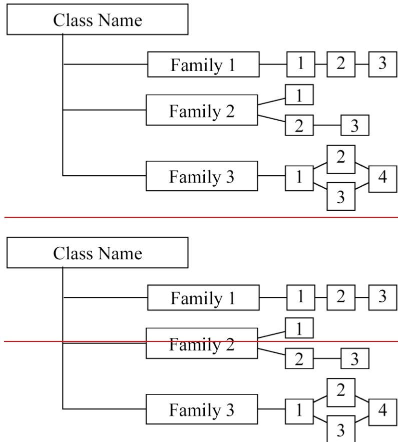
Figure 6 - Sample class decomposition diagram
