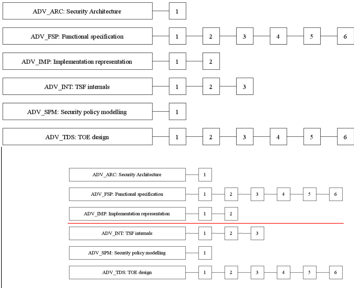
Figure 11 - ADV: Development class decomposition
