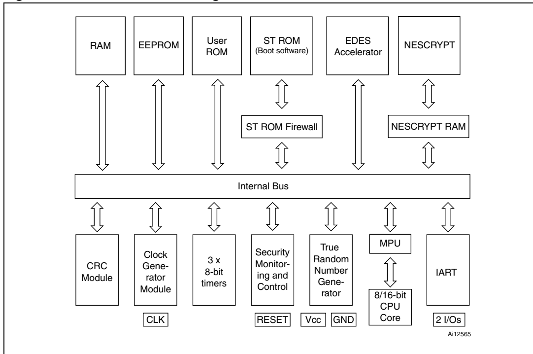
Figure 1. SA23YL80C block diagram
