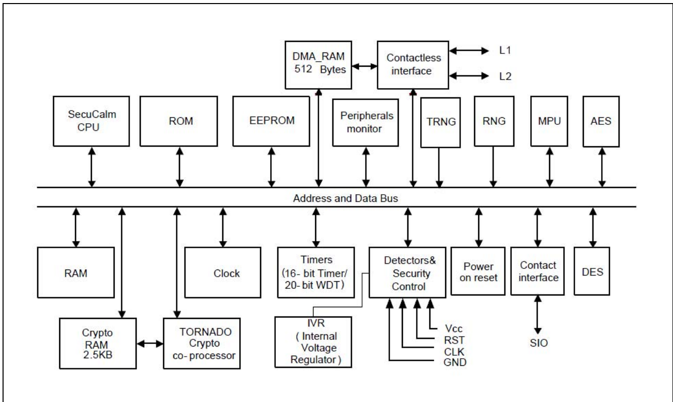
Figure 1. S3CT9KW/S3CT9KC/S3CT9K9 Block Diagram
