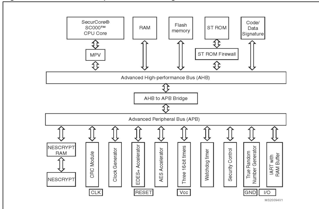
Figure 1. ST31H320 A01 platform block diagram
