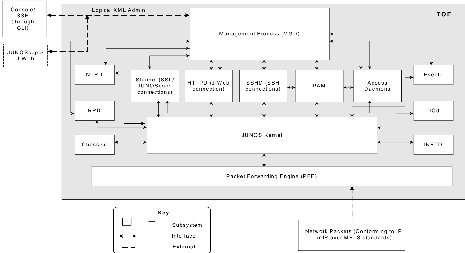
Figure 3: TOE Subsystems
