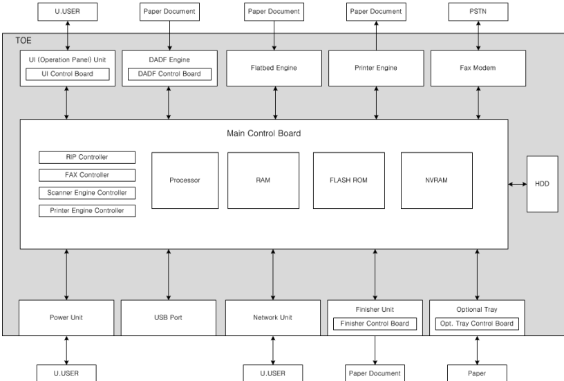
[Figure 2] Physical Structure of MFP
