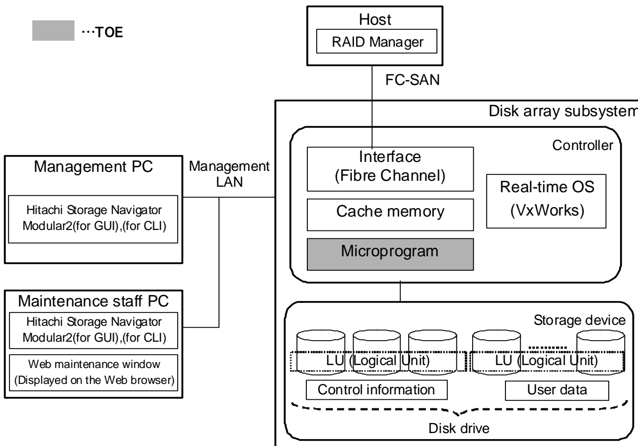
Figure 2 TOE Logical Configuration
