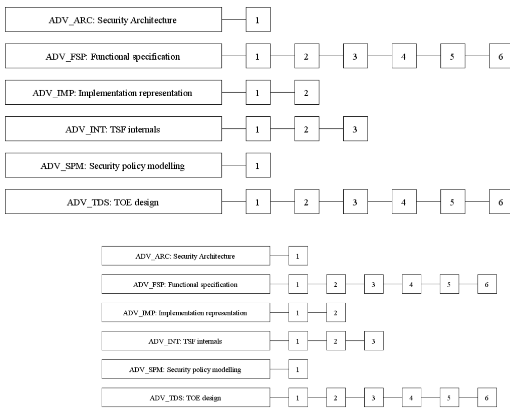
Figure 11 - ADV: Development class decomposition
