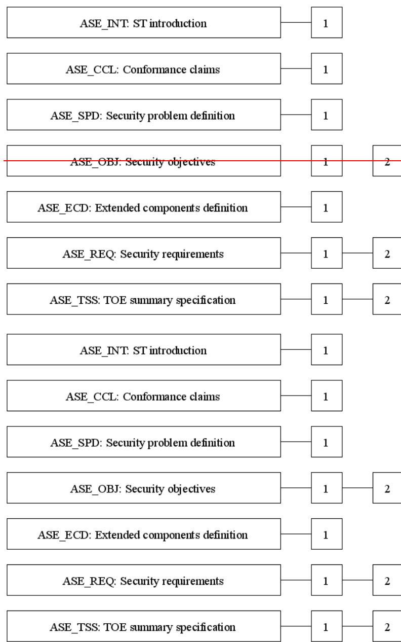
Figure 9 - ASE: Security Target evaluation class decomposition
