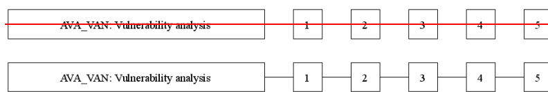
Figure 15 - AVA: Vulnerability assessment class decomposition
