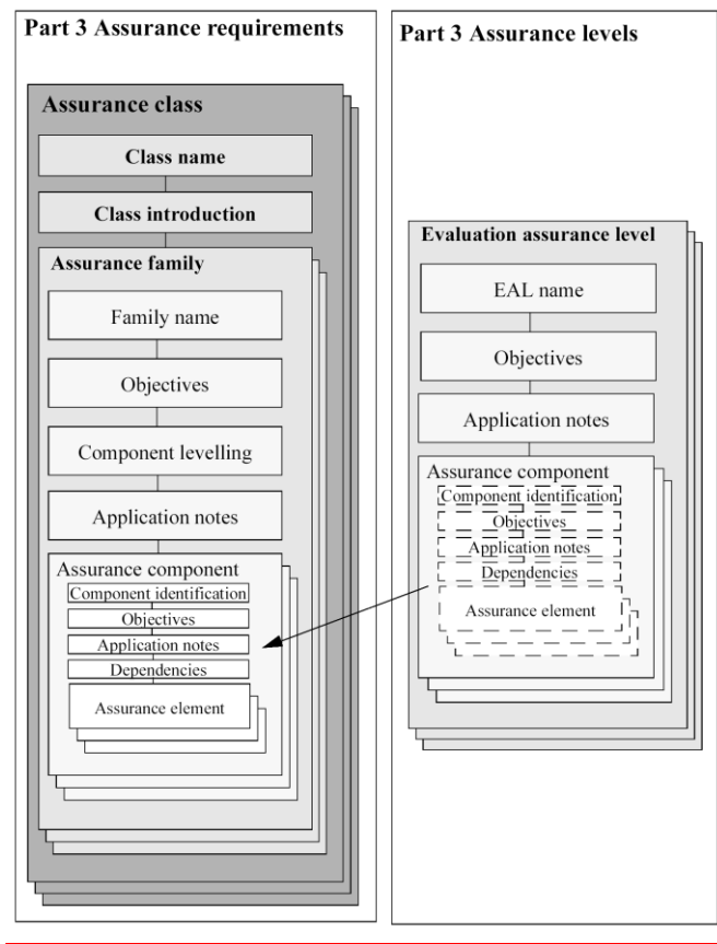
Figure 5 - Assurance and assurance level association
