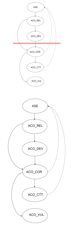
Figure 17 - Relationship between ACO families
