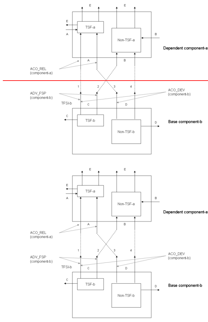
Figure 25 - Composed component interfaces
