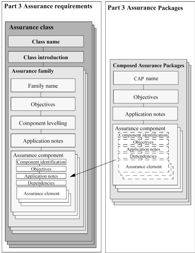
Figure 7 - Assurance and composed assurance package association
