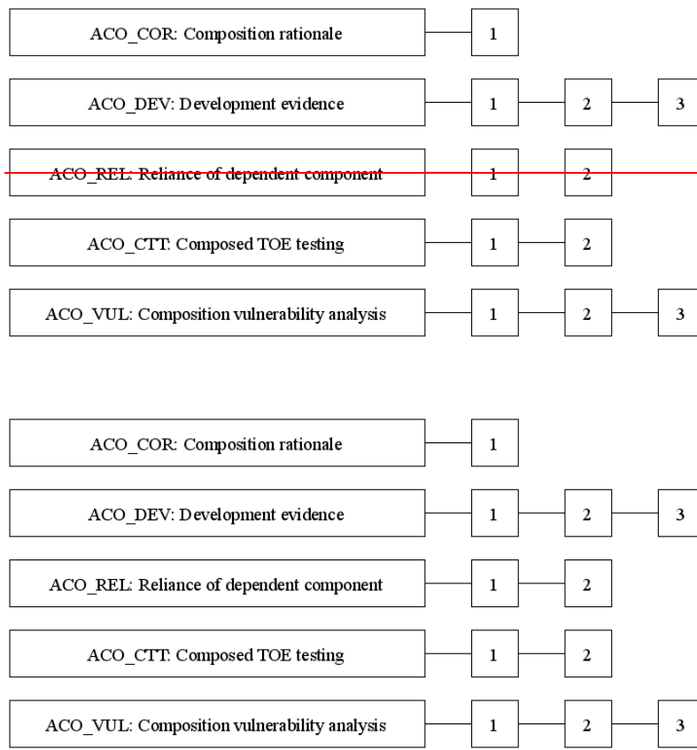
Figure 18 - ACO: Composition class decomposition
