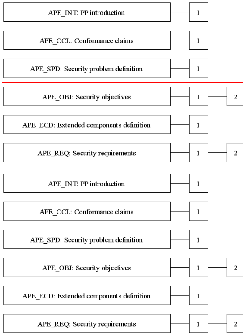
Figure 8 - APE: Protection Profile evaluation class decomposition
