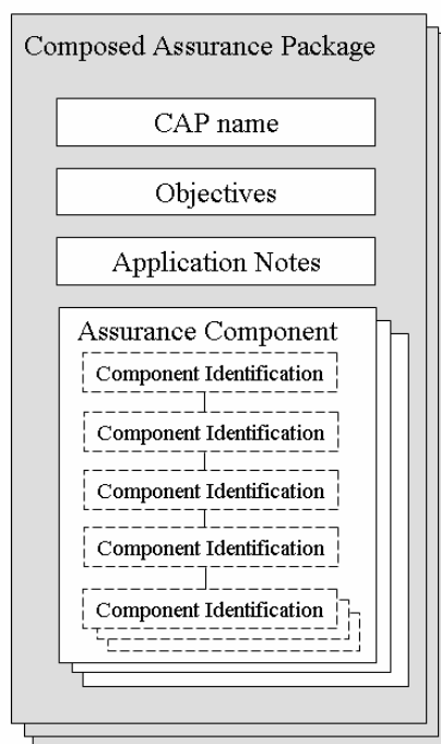
Figure 6 - CAP structure
