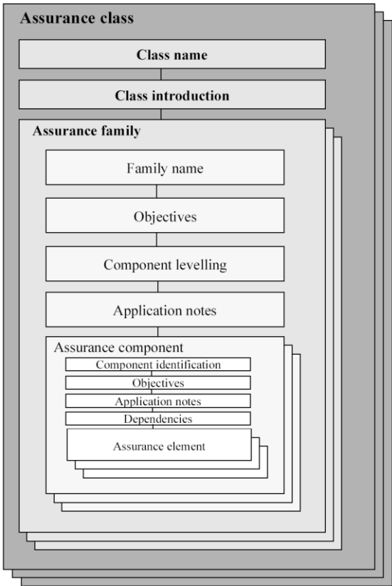
Figure 1 - Assurance class/family/component/element hierarchy
