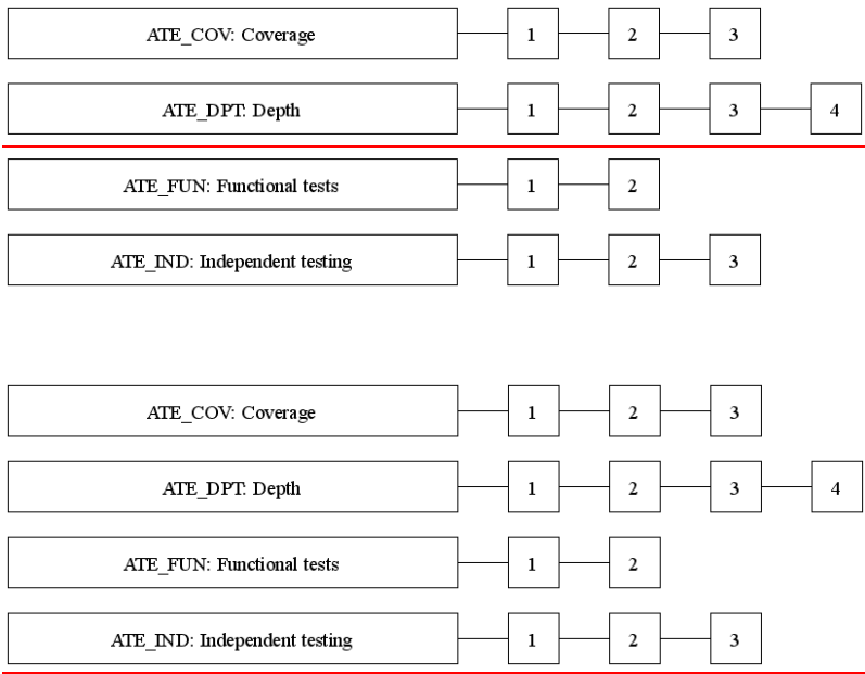
Figure 14 - ATE: Tests class decomposition
