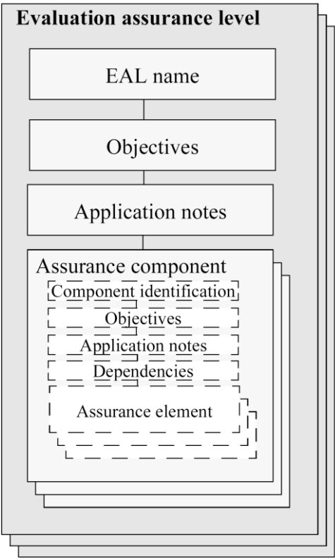
Figure 4 - EAL structure
