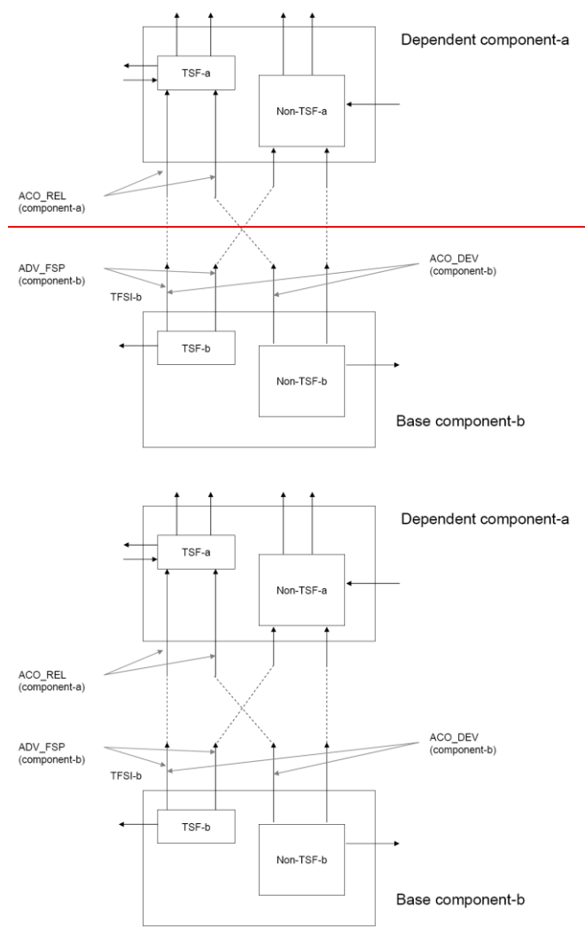
Figure 16 - Relationship between ACO families and interactions between components
