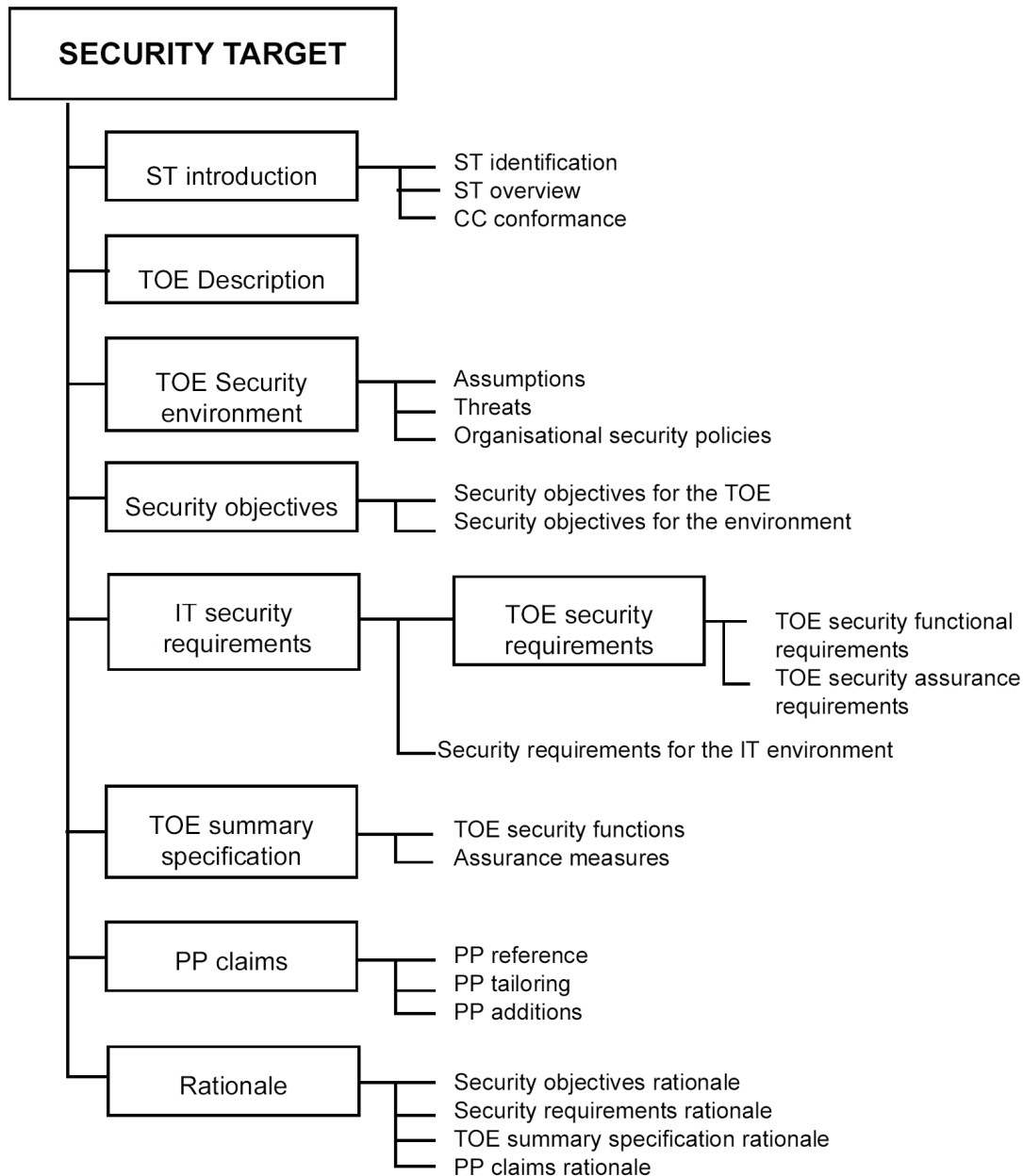
Figure 12 - Security Target content
