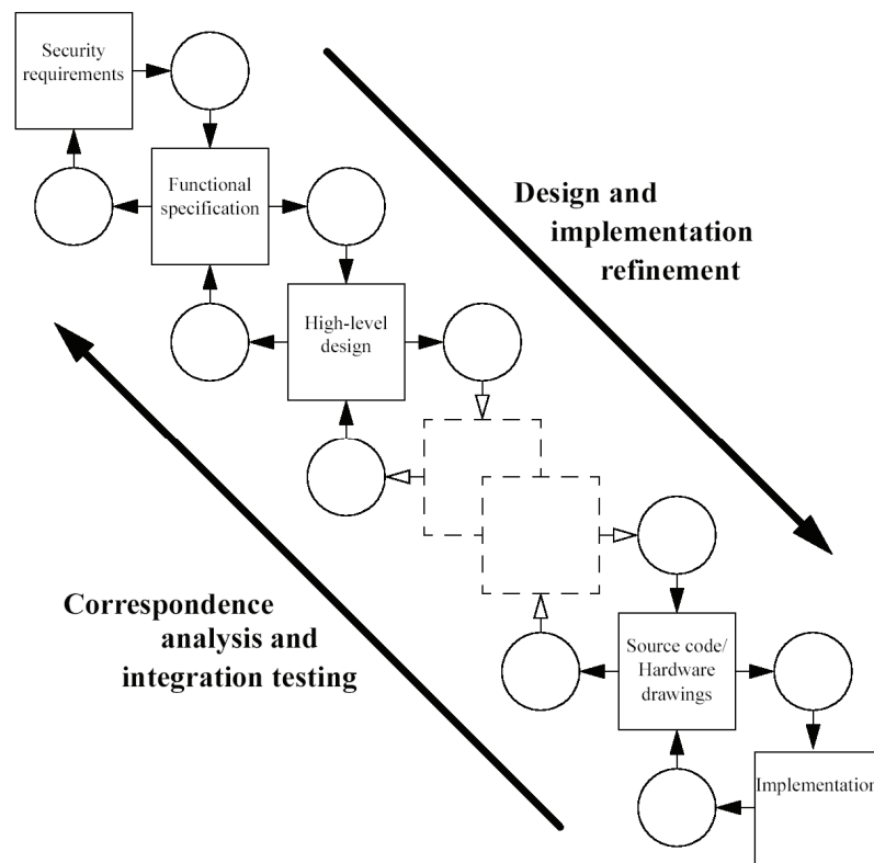
Figure 4 - TOE development model
