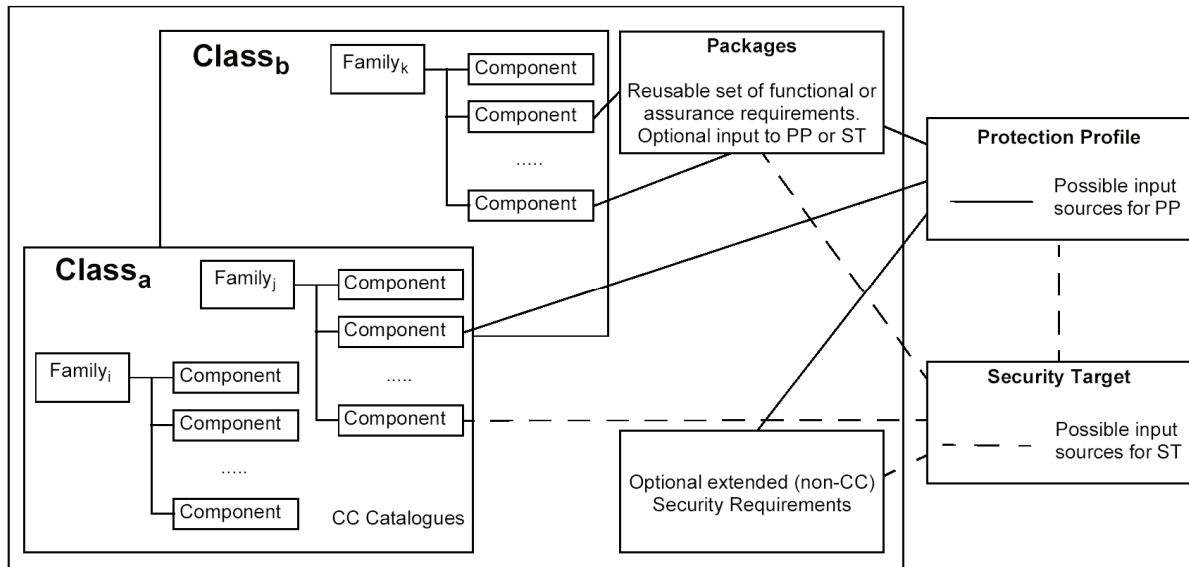
Figure 7 - Organisation and construction of requirements
