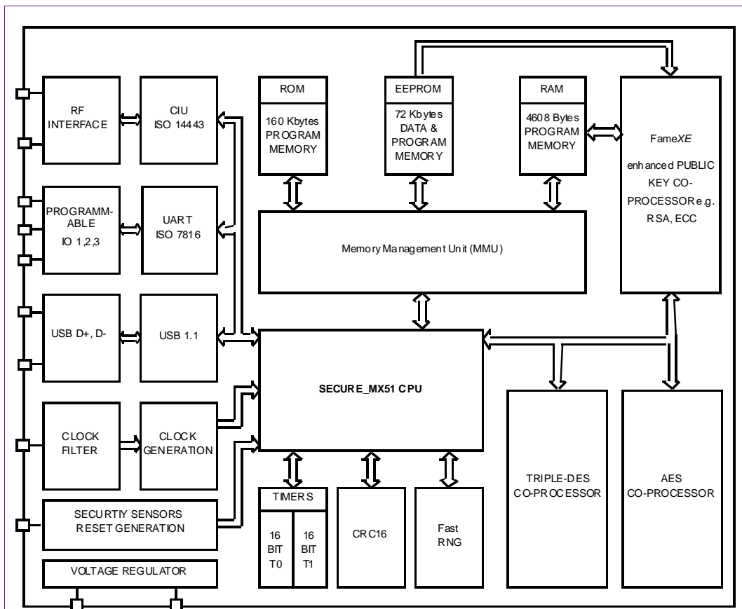
Fig 1. Block Diagram of the P5CT072V0Q
