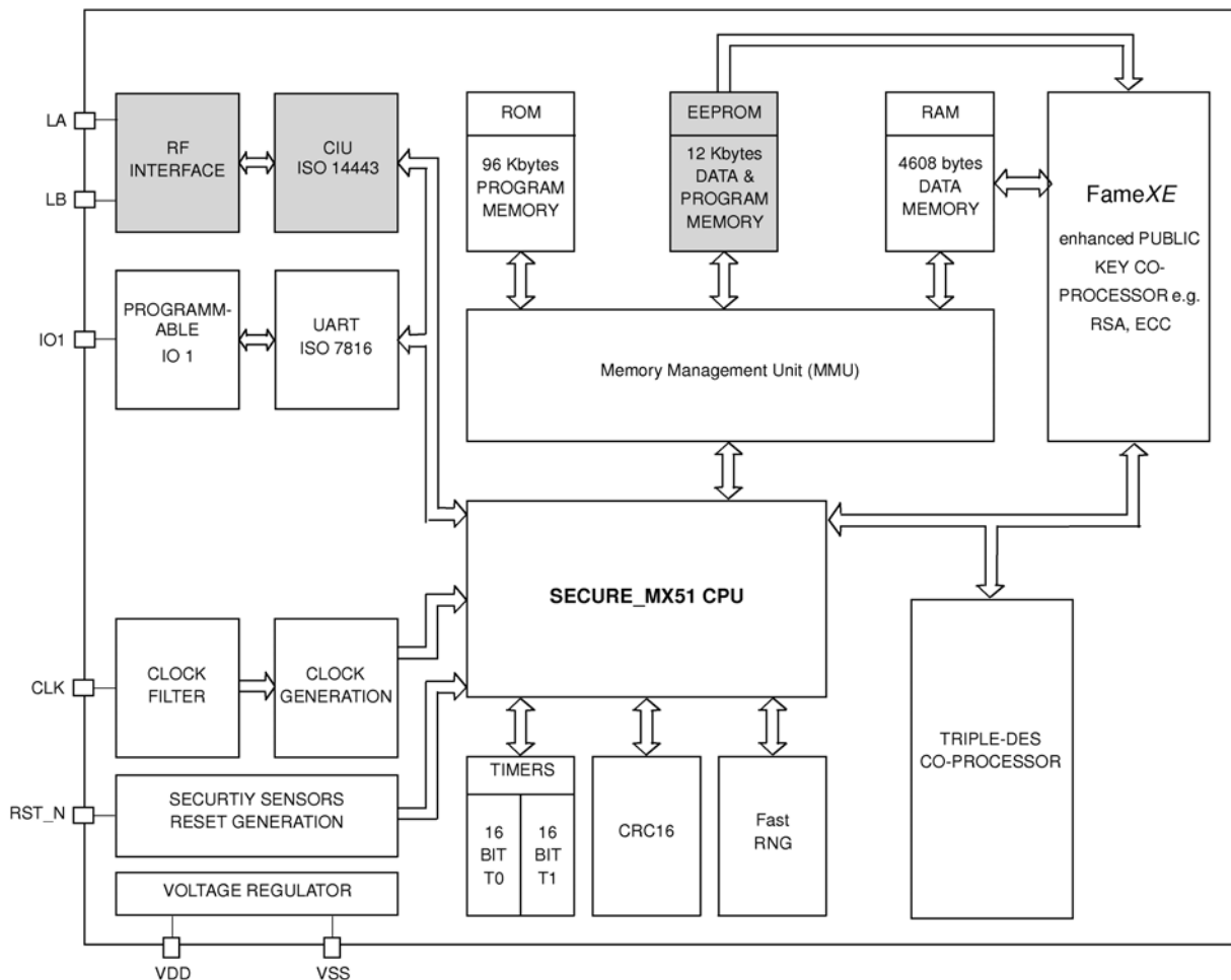
Figure 1: Block Diagram of the P5CD009V2A (grey areas are different for the configurations)
