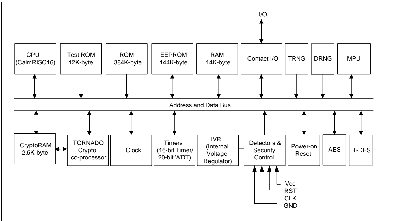
Figure 1. S3CC9PW Block Diagram
