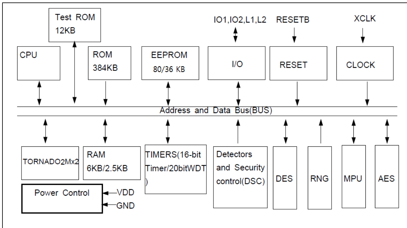
Figure 1. S3CT9KC/S3CT9K9 Block Diagram
