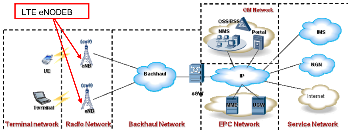
Figure 1 LTE/SAE network
