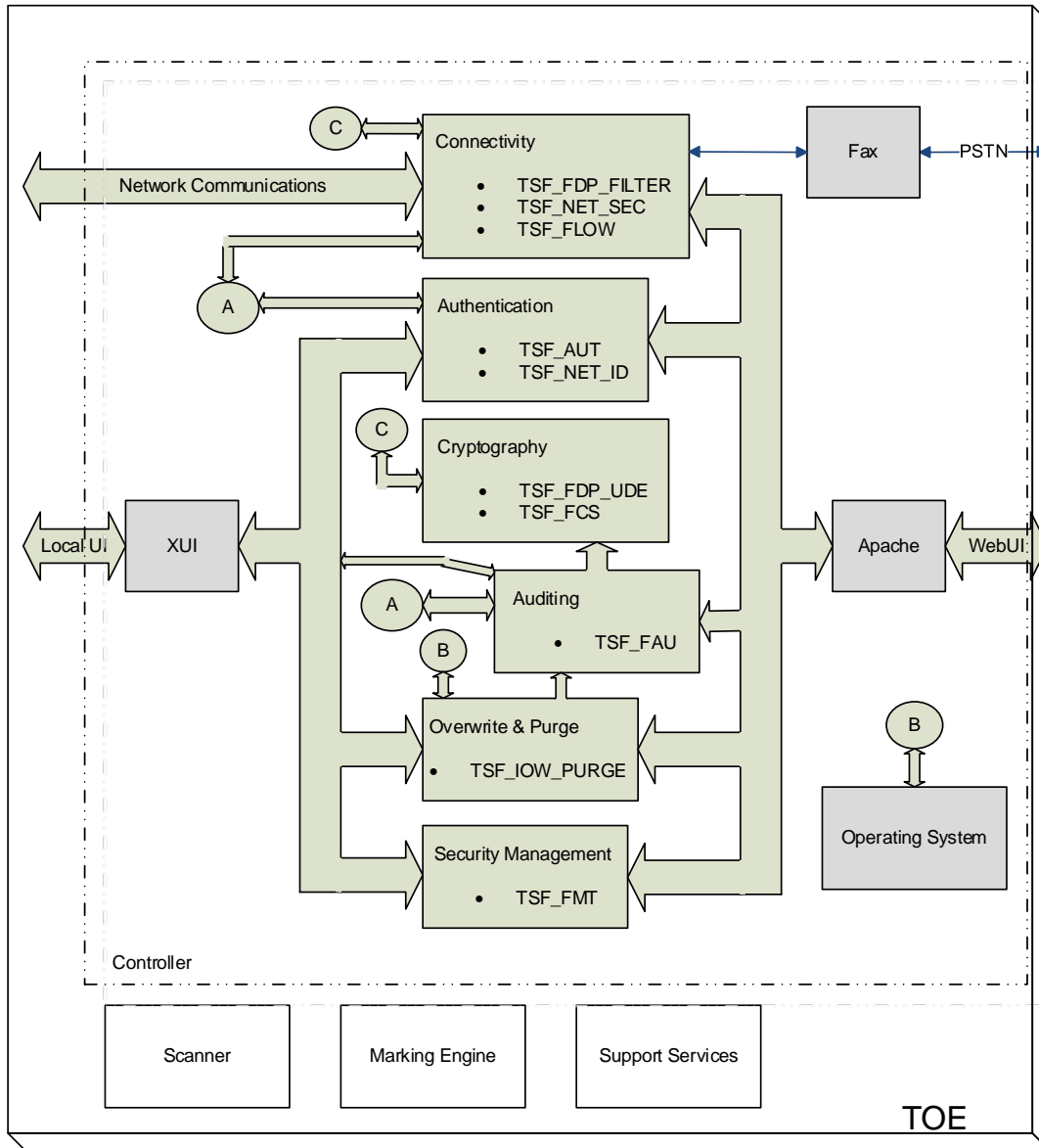
Figure 1 TOE Architecture
