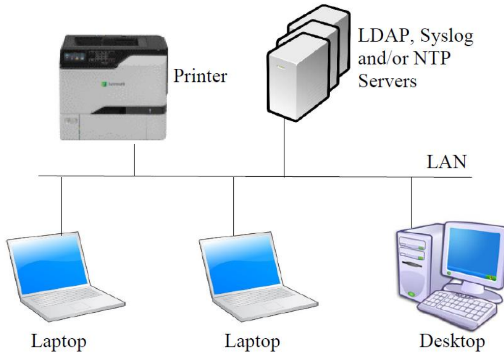
Figure 1 TOE Architecture
