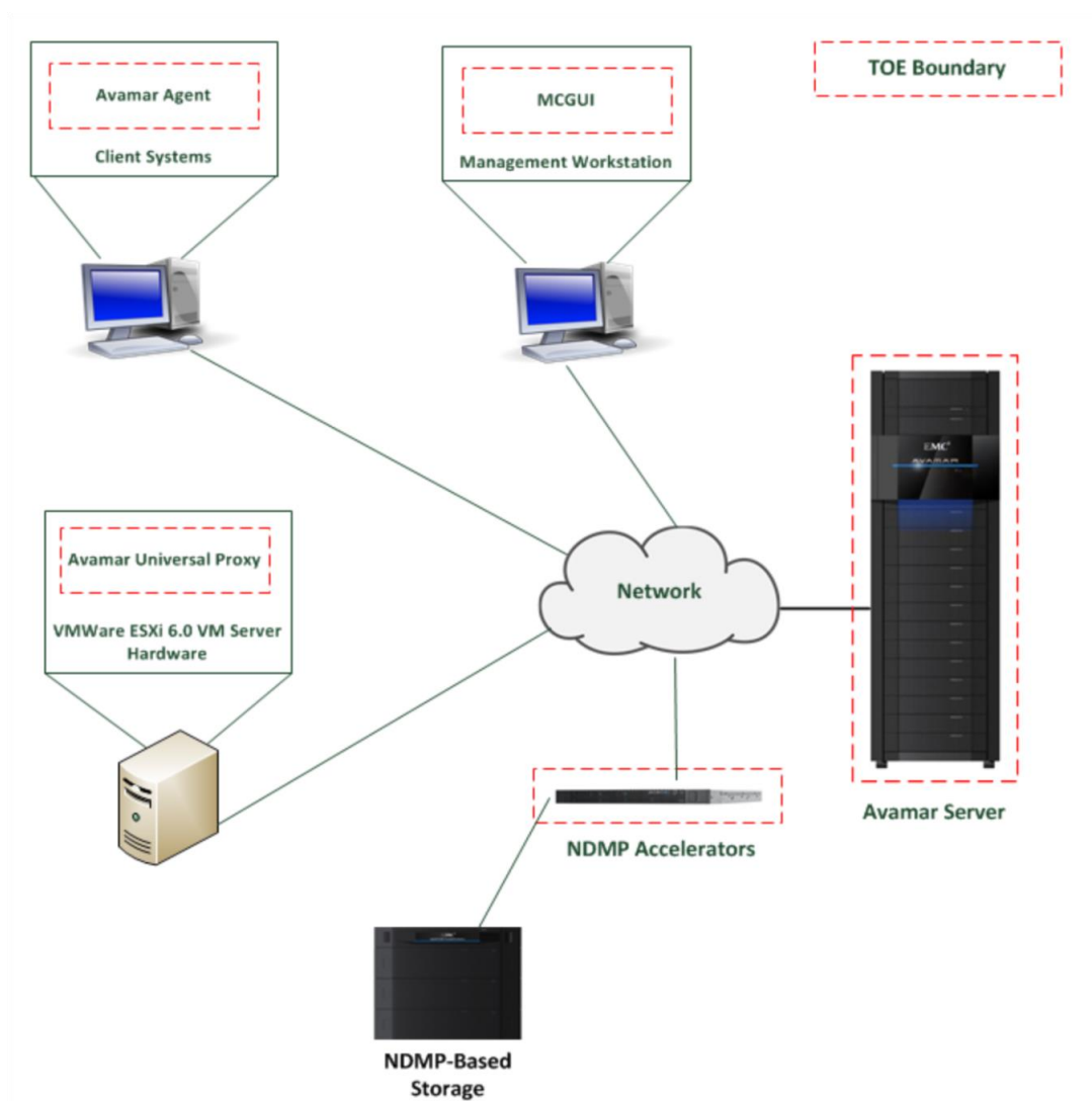
Figure 1: TOE Architecture
