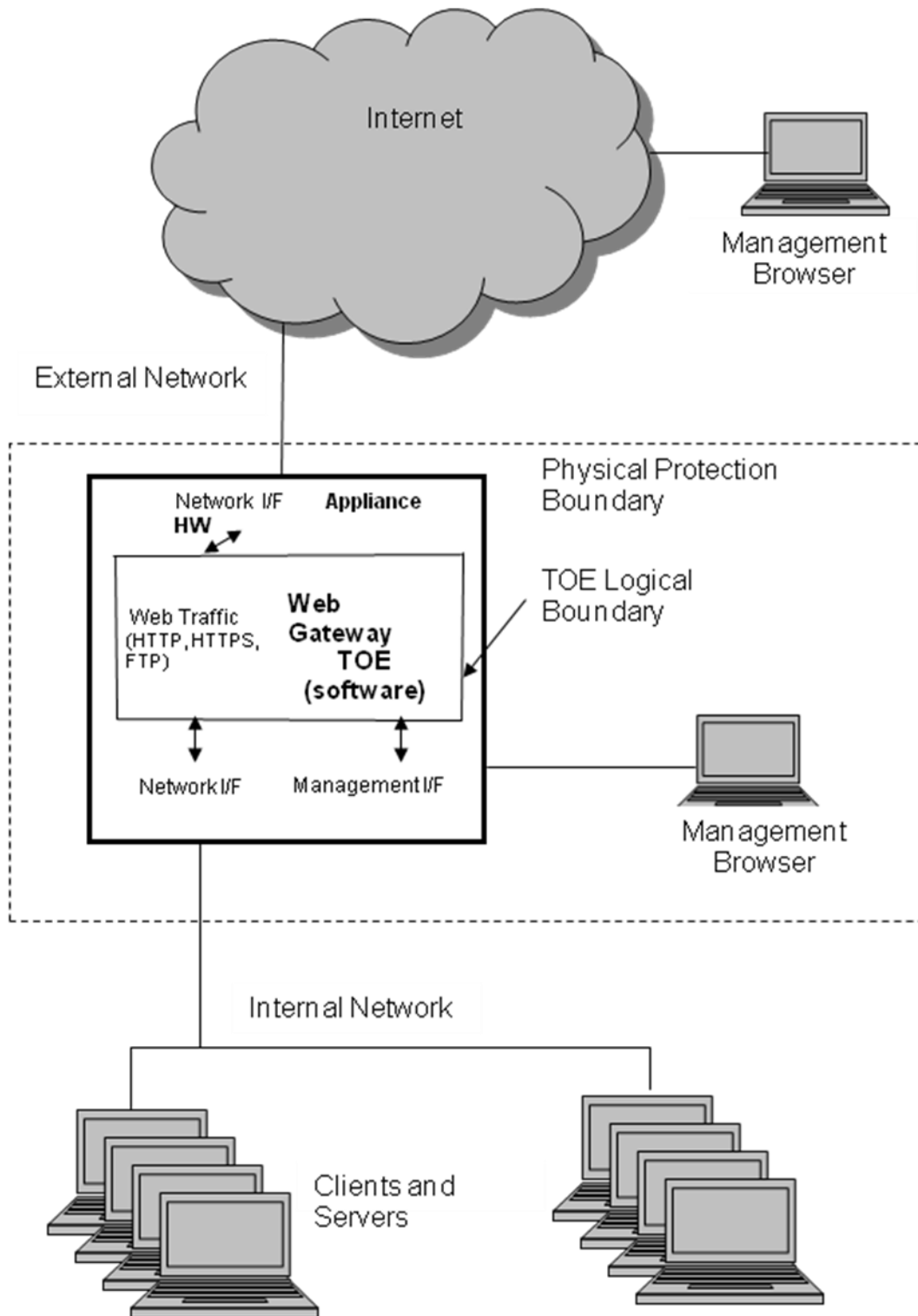
Figure 1 McAfee Web Gateway TOE Security Environment
