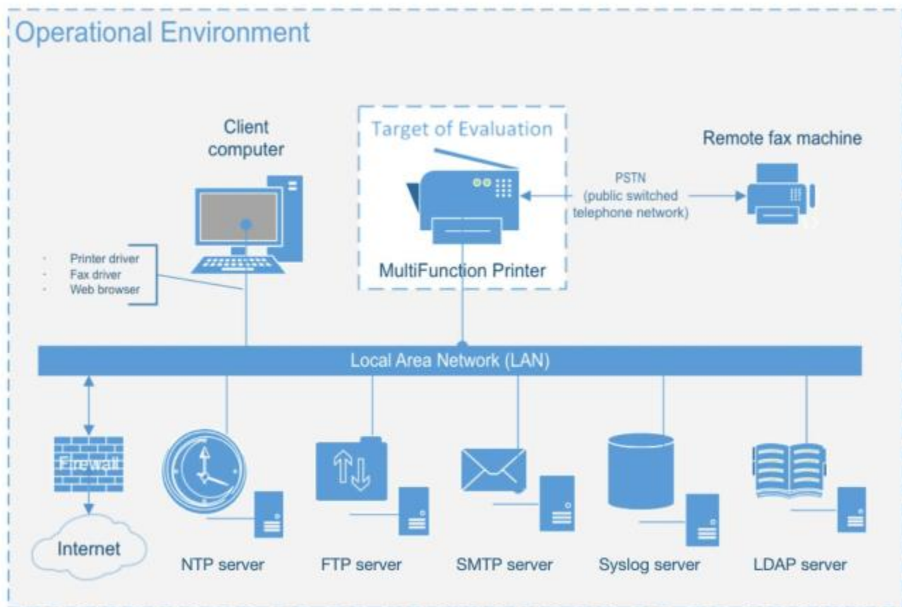
Figure 1: TOE Architecture
