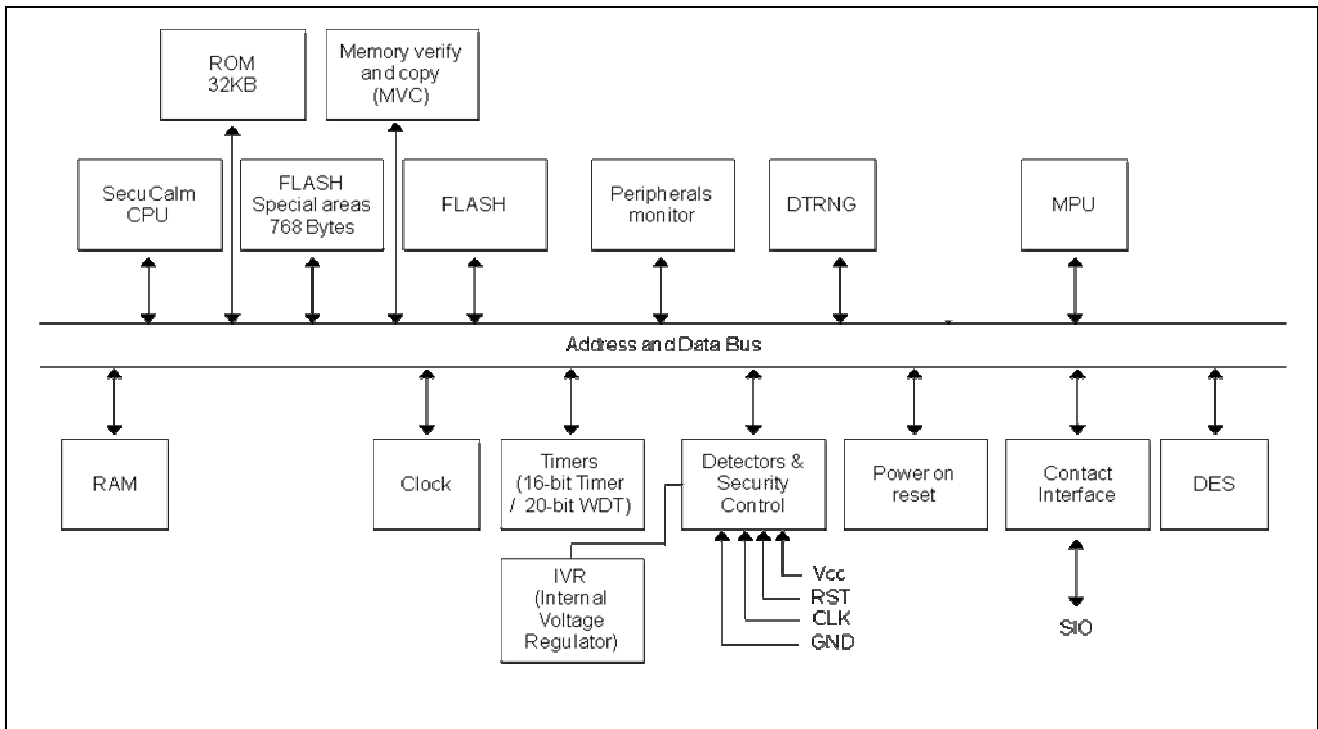
Figure 1. S3FT9FD/ S3FT9FC/ S3FT9FB Block Diagram
