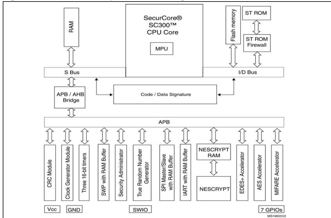
Figure 1. ST33G1M2 D02 platform block diagram
