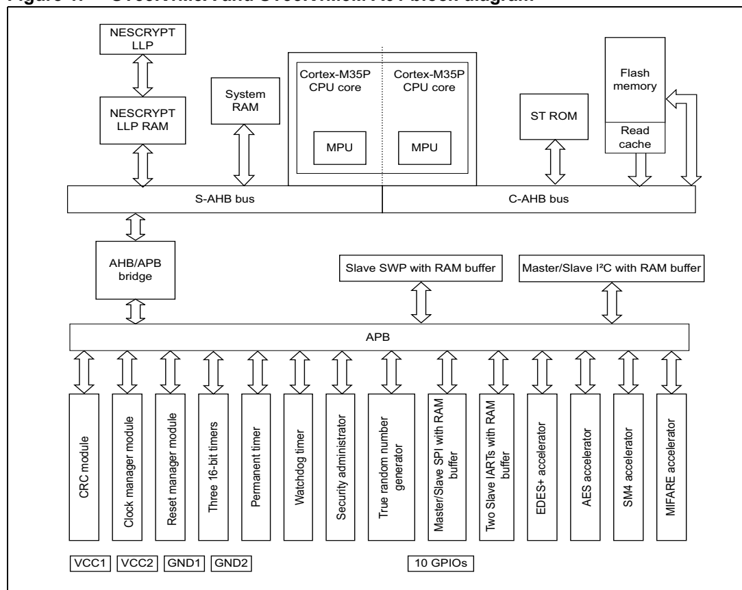
Figure 1. ST33K1M5A and ST33K1M5M A01 block diagram
