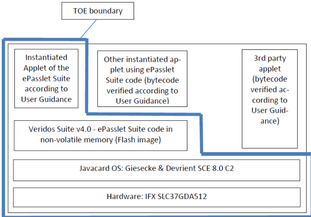
Figure 1 TOE components.
