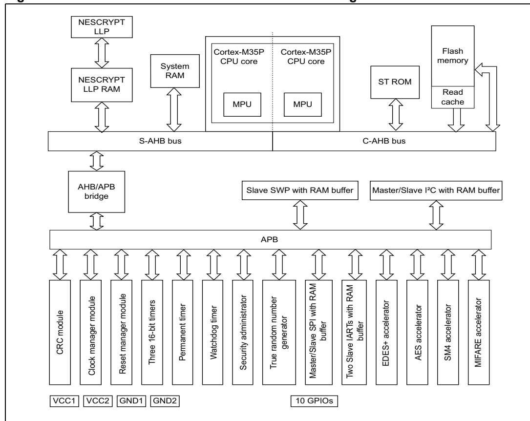
Figure 1. ST33K1M5A and ST33K1M5M B01 block diagram
