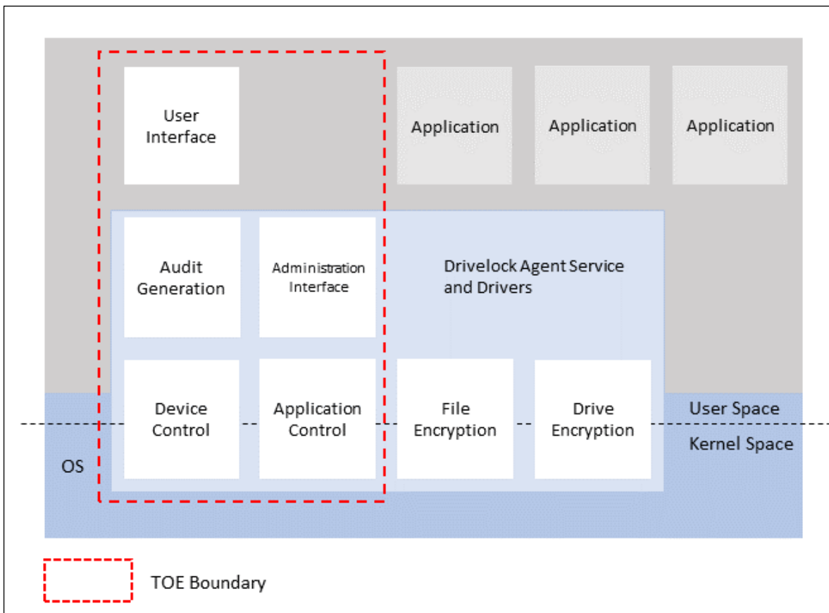
Figure 2 – Overview of the TOE and its environment
