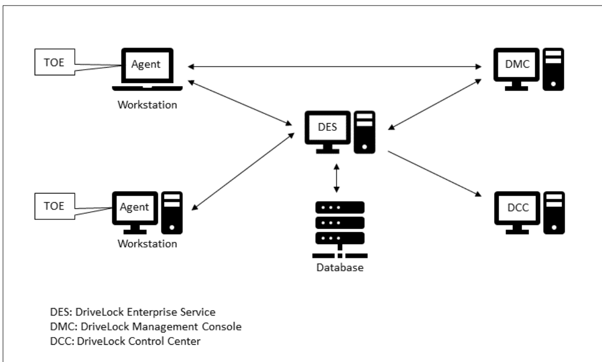
Figure 1 – Overview of TOE installation and environment
