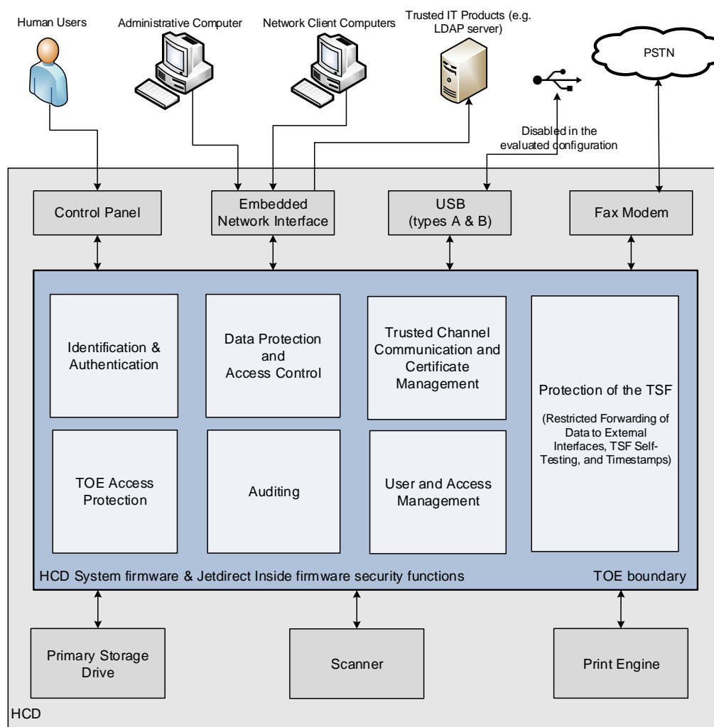
Figure 2: HCD Logical Scope Diagram
