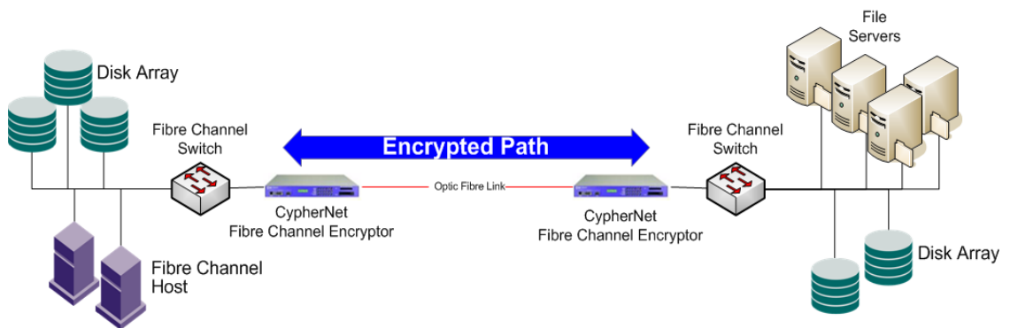
Figure 3 – Fibre Channel Security Solution
