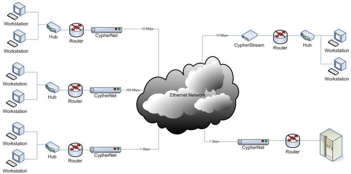
Figure 2 – Ethernet Security Solution
