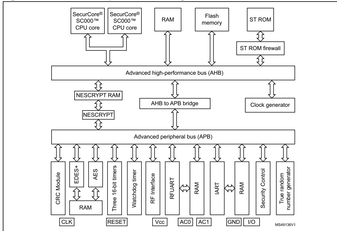
Figure 1. ST31P450 B05 platform block diagram
