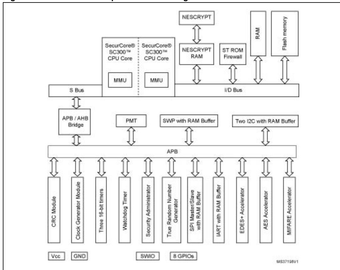
Figure 1. ST33J2M0 B02 platform block diagram
