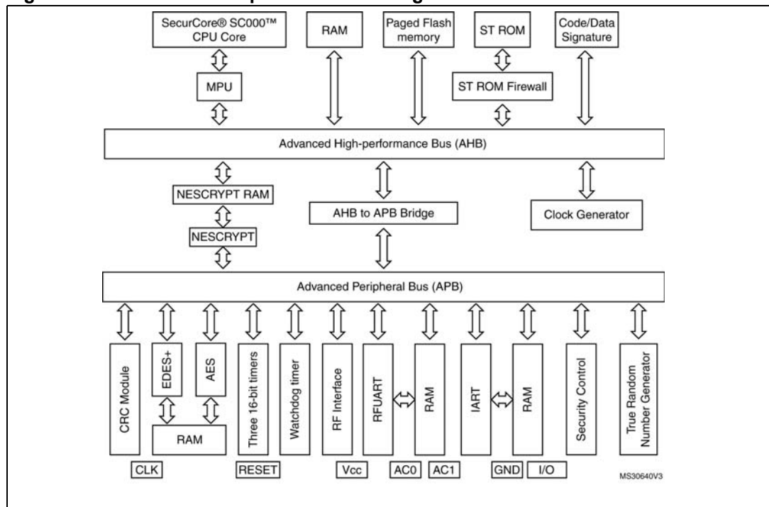
Figure 1. ST31G480 E05 platform block diagram
