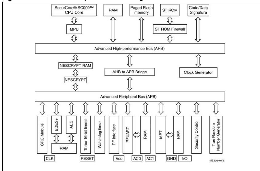
Figure 1. ST31G480 E01 platform block diagram
