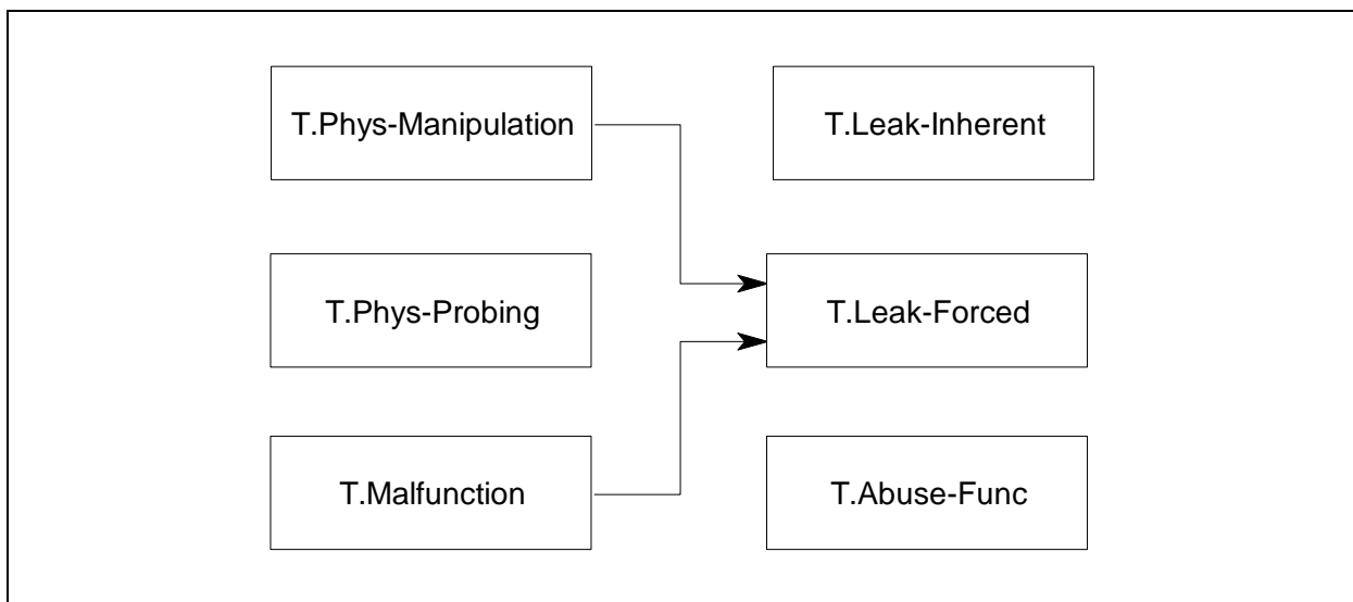
Figure 3: Standard Threats
