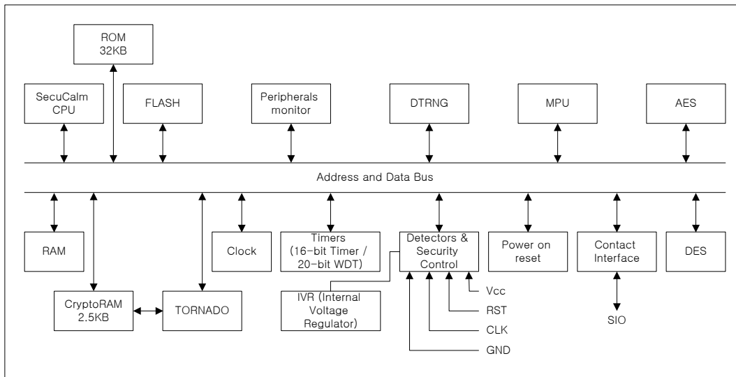
Figure 1. S3FT9PF/S3FT9PT/S3FT9PS Block Diagram
