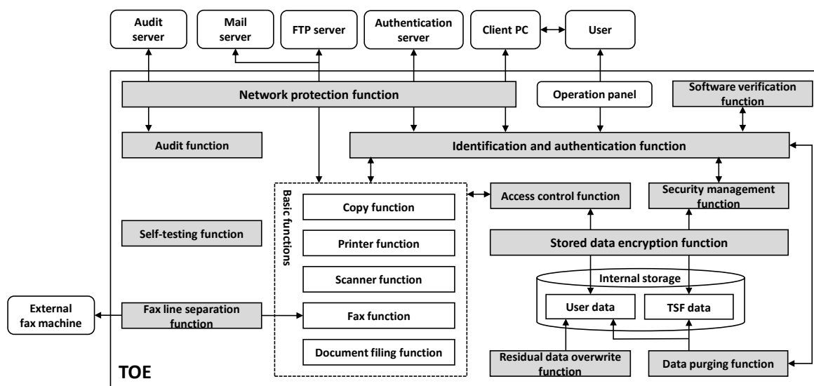
Figure 5-1 TOE boundary
