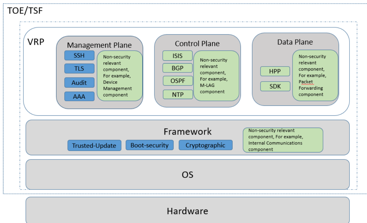
Figure 2 Architecture and boundaries of the Target of Evaluation
