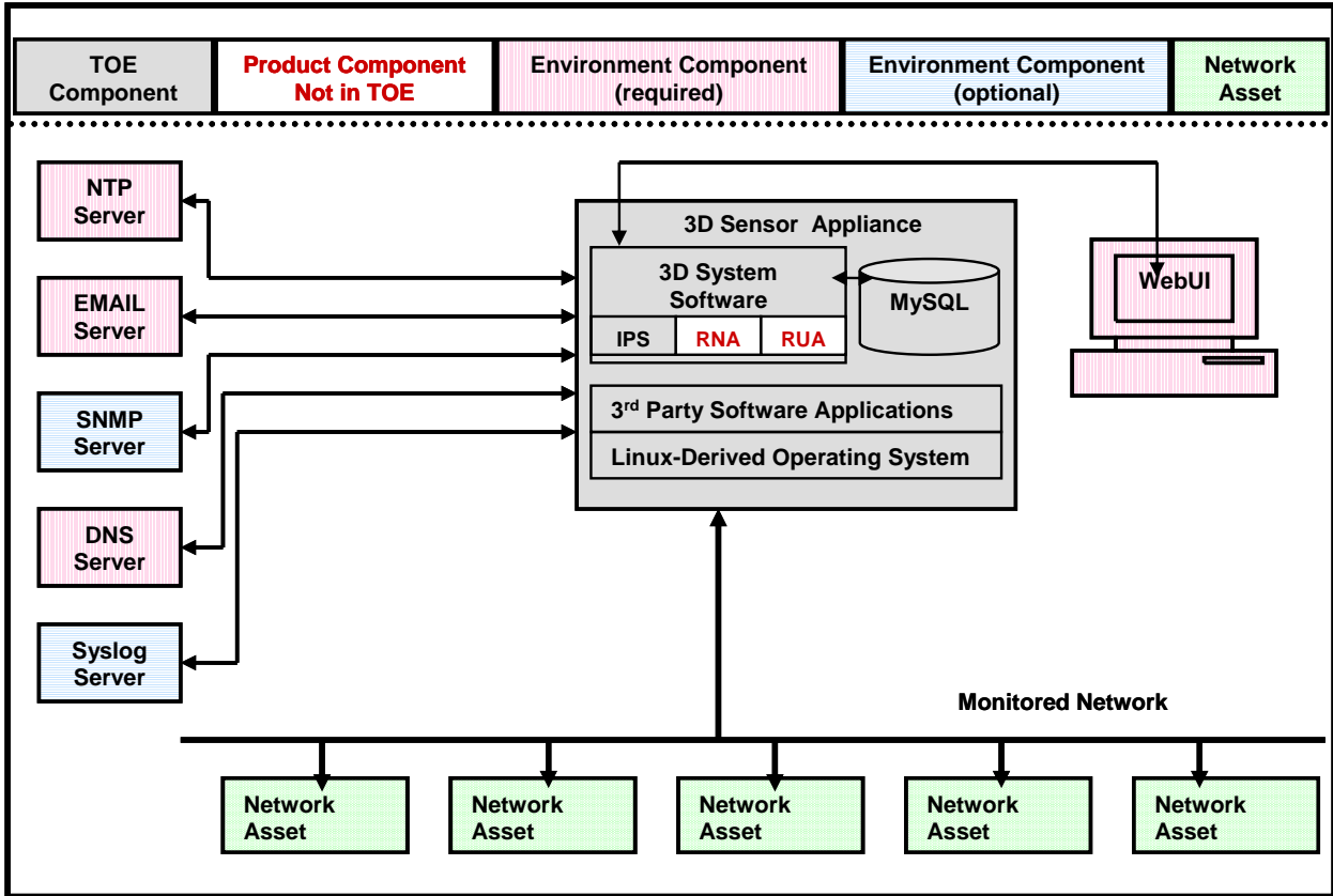
Figure 2: Sourcefire 3D System using a stand-alone 3D Sensor with IPS
