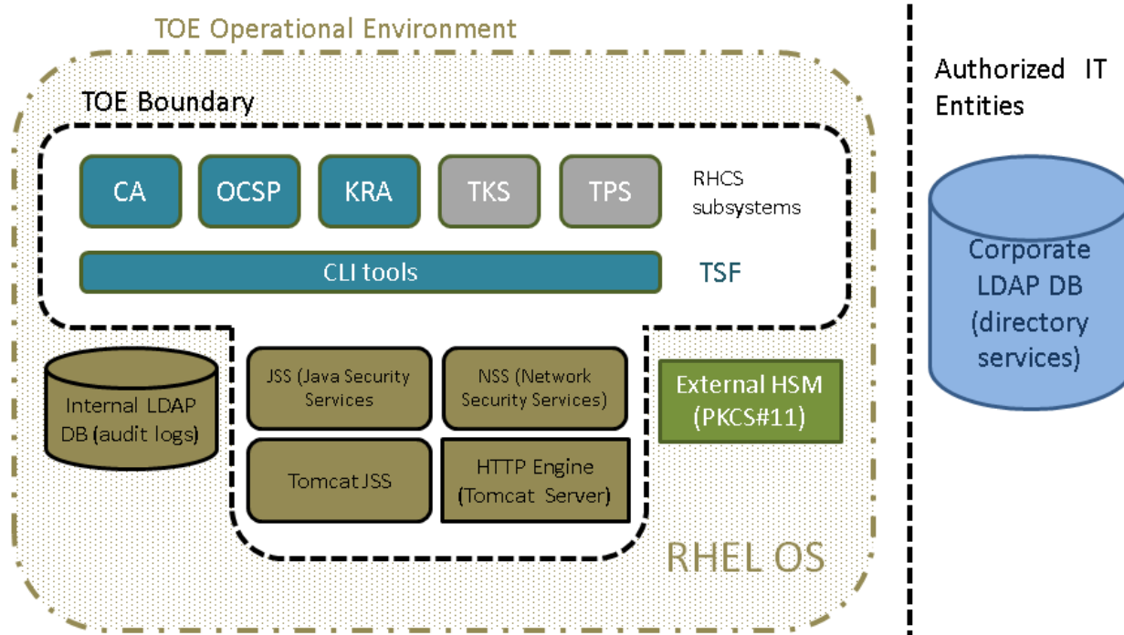
Figure 1-1 RHCS System Architecture
