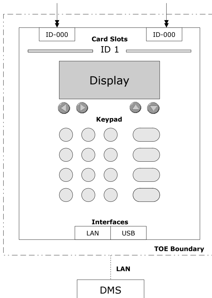
Figure 2: TOE Boundary
