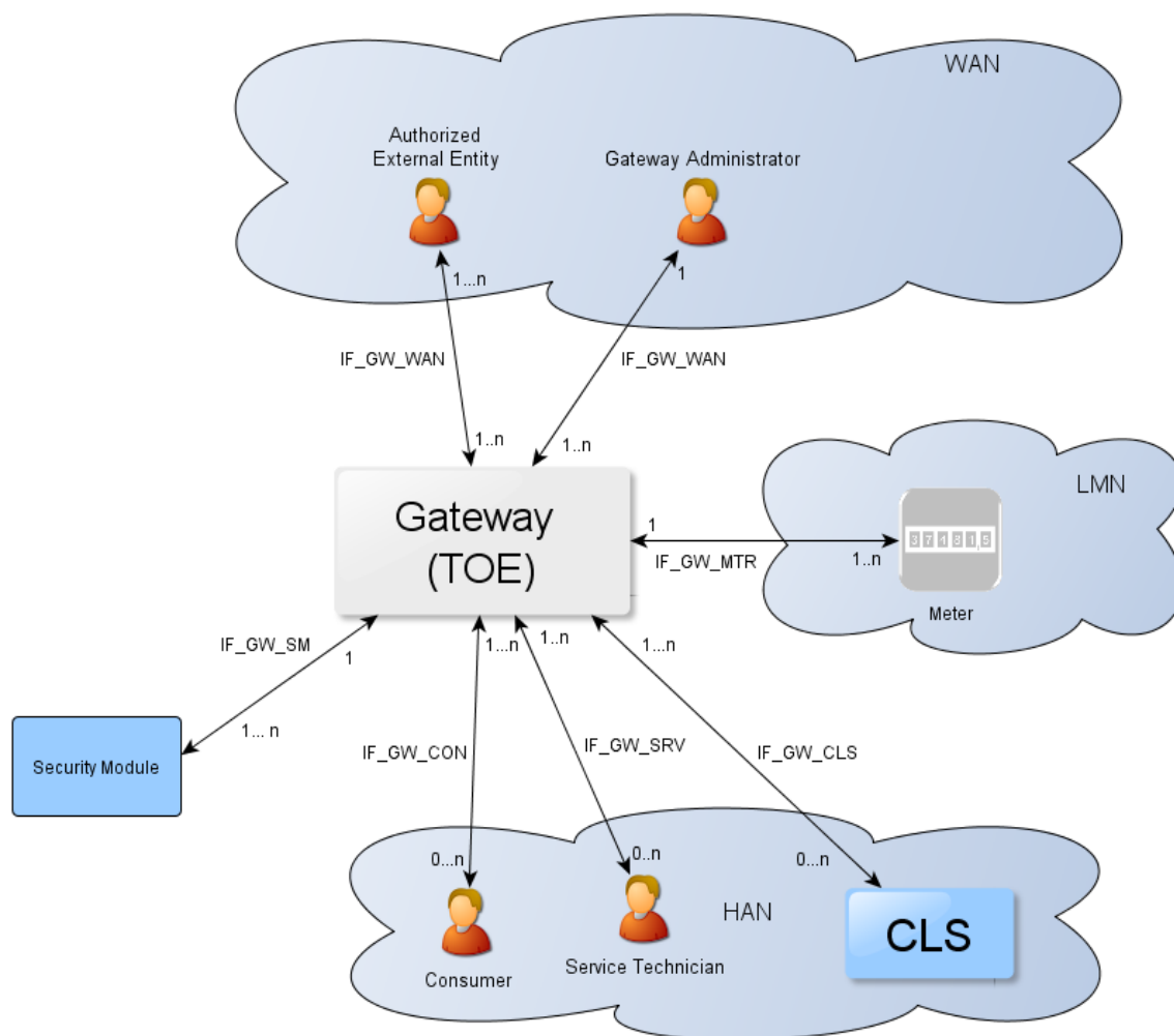
Figure 2: The logical interfaces of the TOE 14
