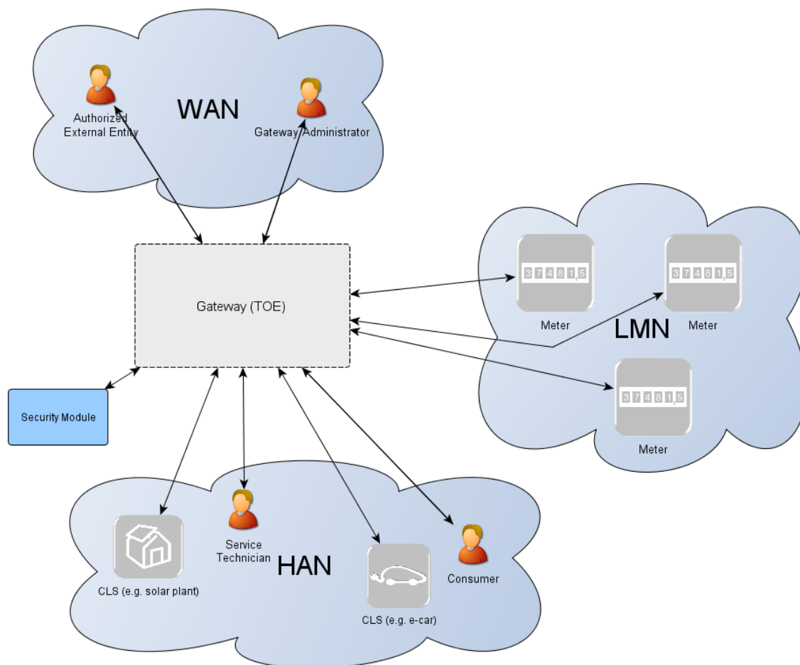
Figure 1: The TOE and its direct environment 9
