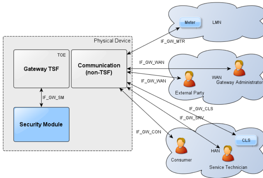
Figure 3: General design of the product 27
