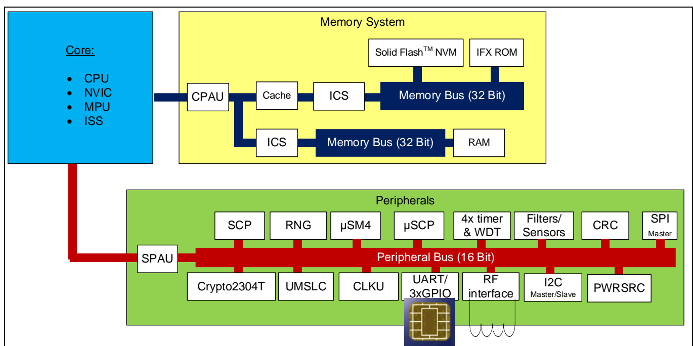
Figure 1 Block diagram of TOE hardware
