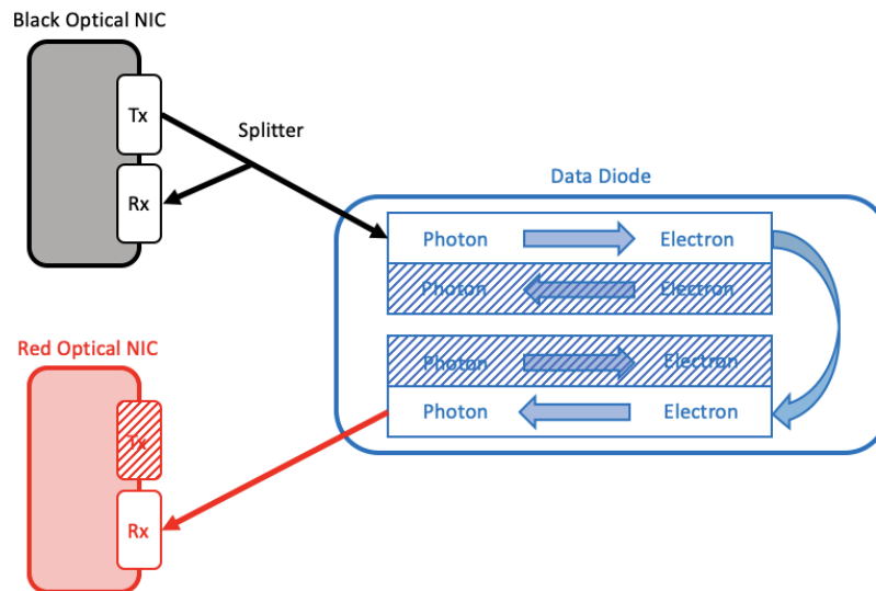
Figure 22: Data Diode Connectivity
