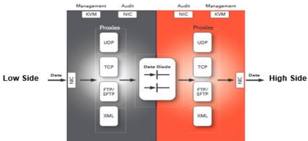
Figure 22: Data Diode Connectivity
