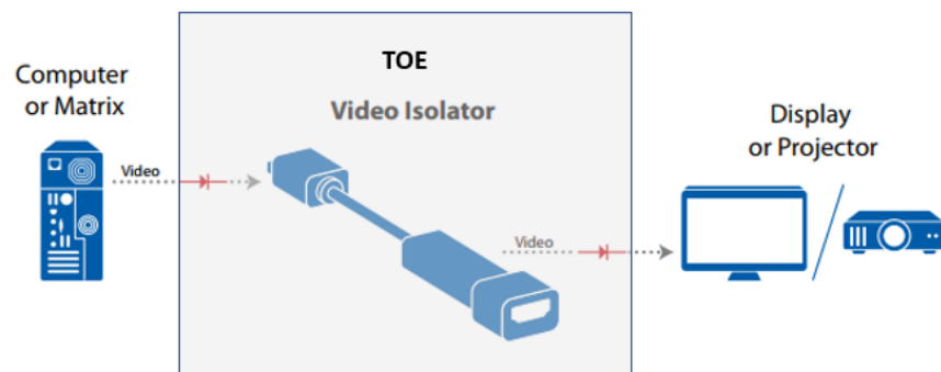
Figure 2: TOE Architecture - Mini Isolator
