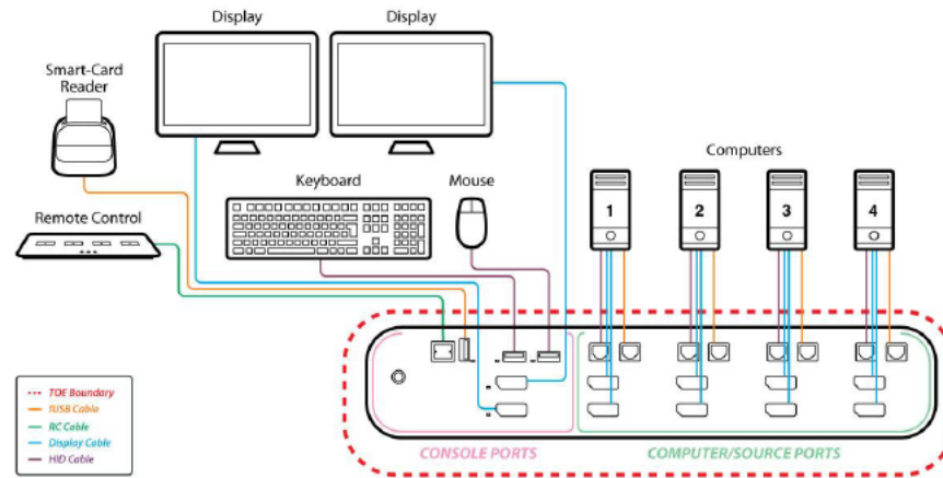
Figure 1: TOE Architecture
