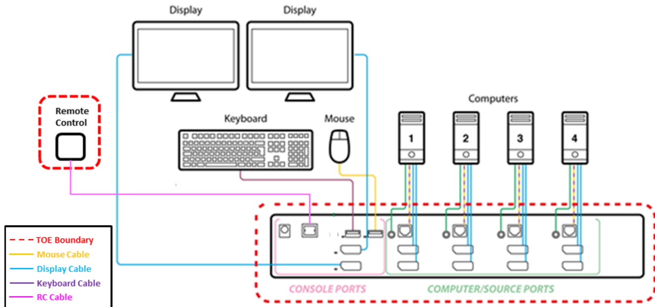
Figure 1: TOE Architecture
