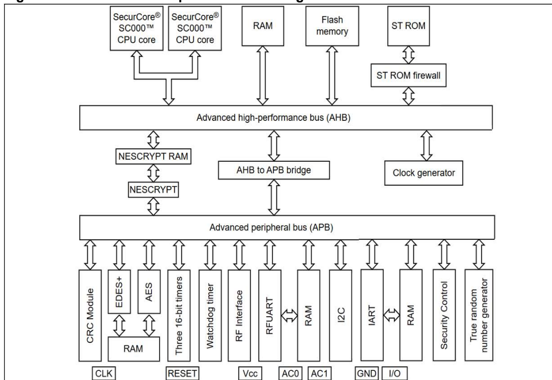
Figure 1. ST31R480 B02 platform block diagram
