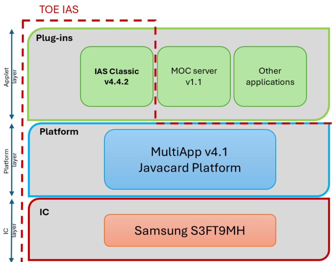
Figure 1: TOE Boundaries
