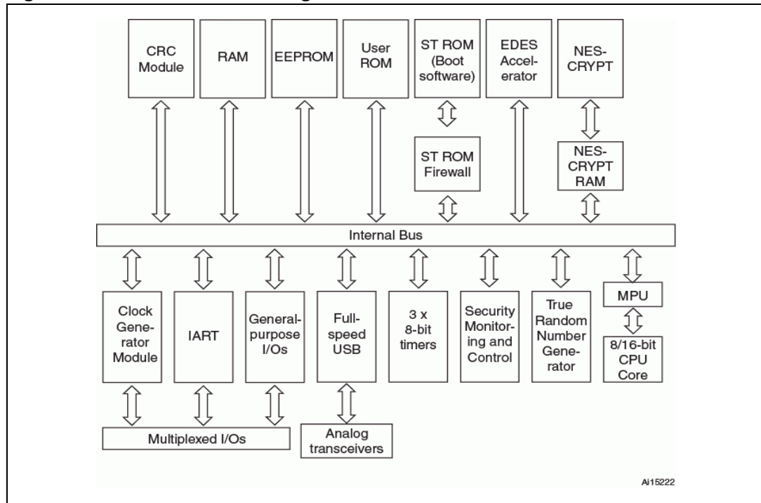
Figure 2. Sx23YT34A block diagram
