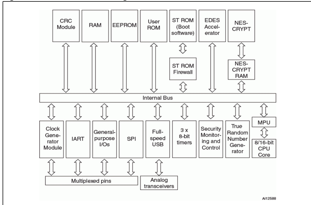
Figure 1. Sx23YT66A block diagram
