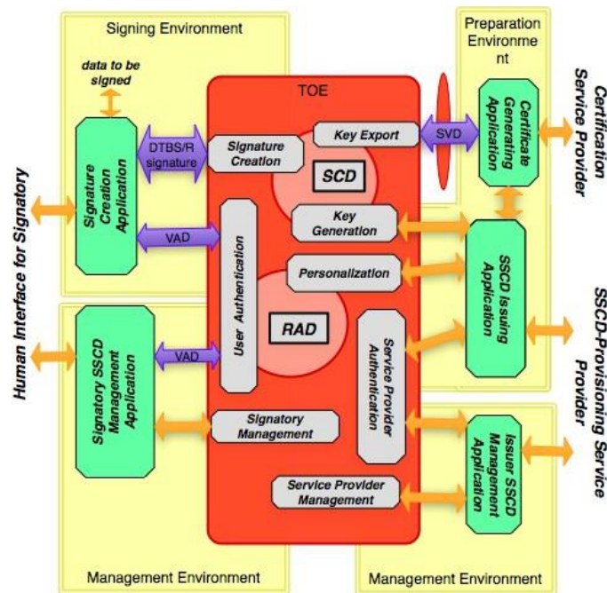
Figure 5: TOE and Operational environments with Key Generation and trusted channel to CGA
