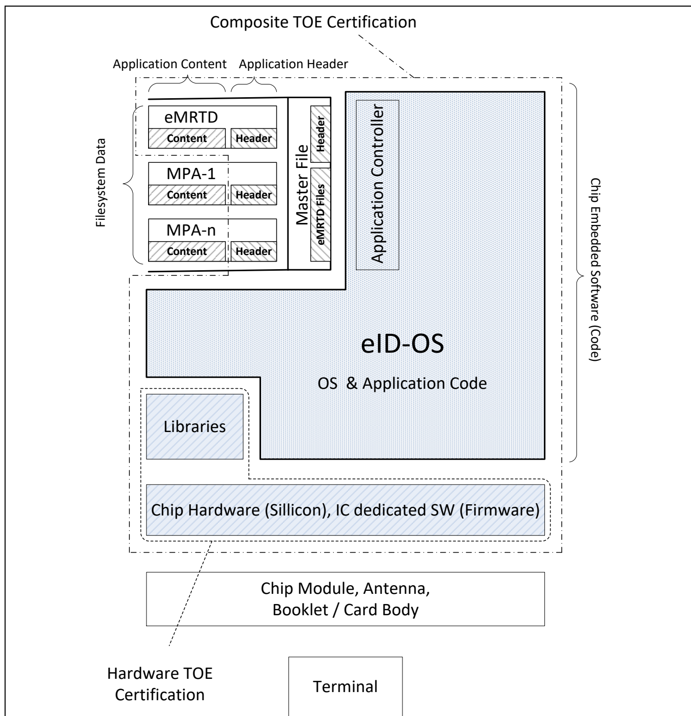
Figure 1 TOE block diagram
