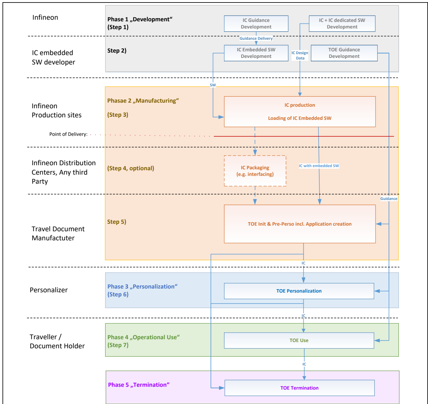
Figure 2 TOE life-cycle
