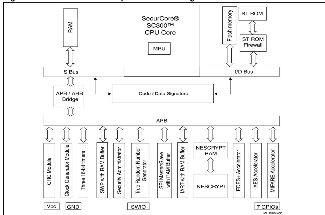
Figure 1. ST33G1M2AM D03 platform block diagram
